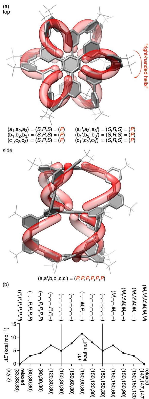
Fig. 4. Structure of phenine dipolluxene ( 1 ). (a) Crystal structure. A representative structure of the (P, P, P, P, P, P) -isomer is shown. The mirror-image enantiomer, (M, M, M, M, M, M) , was also found in the crystal of the racemate (Fig. S4). (b) Energetics of the conformers, showing an energy barrier of ~11 kcal
