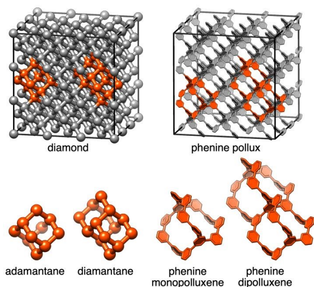
Fig. 1. Strongly isotropic nets of carbon atoms. (a) Diamond and its molecular segments (adamantane and diamantane). (b) Phenine pollux and its molecular segments (monopolluxene and dipolluxene).
