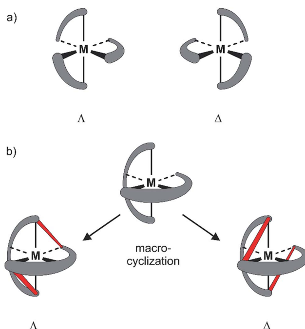
Fig. 1 Sketch of axial chirality in metal complexes: (a) axial chirality with bidentate ligands (e.g. 2,2'-bipyridine). (b) Concept of introducing chirality by macrocyclization. Top: achiral complex of a tridentate ligand (e.g. 2,2':6',2''-terpyridine). Bottom: axial chiral metal complexes obtained by interlinking the ends of the two tridentate ligands (interlinking bridges in red).
