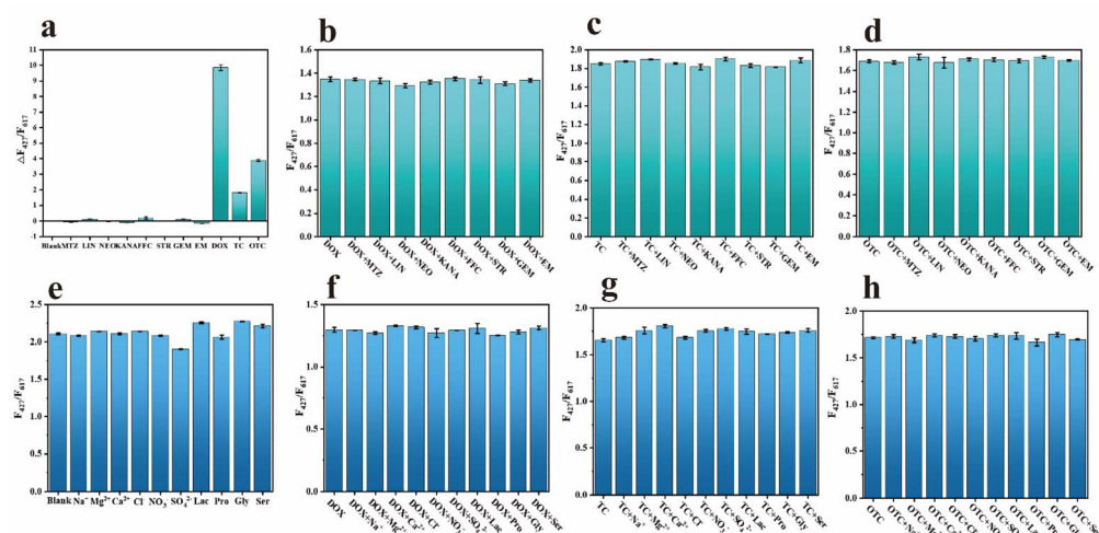
Fig. 6 Selectivity detection of \text{NH}_2\text{-BDC-Eu-DPA} (a); detection of DOX (b), TC (c), and OTC (d) in the presence of other antibiotics. Anti-interference analysis of \text{NH}_2\text{-BDC-Eu-DPA} (e); detection of DOX (f), TC (g), and OTC (h) in the presence of interfering substances.
