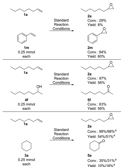
Scheme 2 Competitions experiments of 1-octene with selected other substrate classes. Conversion and yield determined by GC analysis with hexadecane as IST. a MeCN:H 2 O (95 : 5) as solvent.
