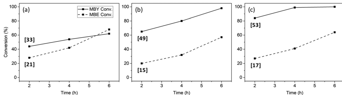
Fig. 9 Conversion of MBY and MBE for (a) 10Ni/Ti-M 500 , (b) 10Ni/Ti-A 500 , and (c) 10Ni/Ti-R 500 catalysts. The numbers in square brackets represent TON at 2 h. Reaction conditions: reactant – 1 g, H 2 O – 40 g, catalyst – 100 mg, temp. – 30 °C, time – 2–6 h, H 2 – 10 bar (at 30 °C), and RPM – 900.
