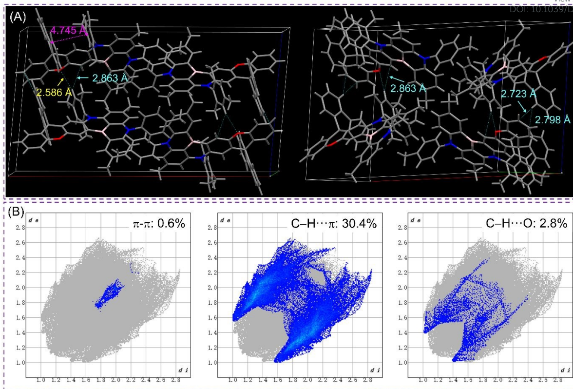
Fig. 2. (A) Packing patterns characterized by abundant C-H... \pi and C-H...O bonds and (B) the primary intermolecular interactions along with their respective proportions in SFX-3BN crystal.
