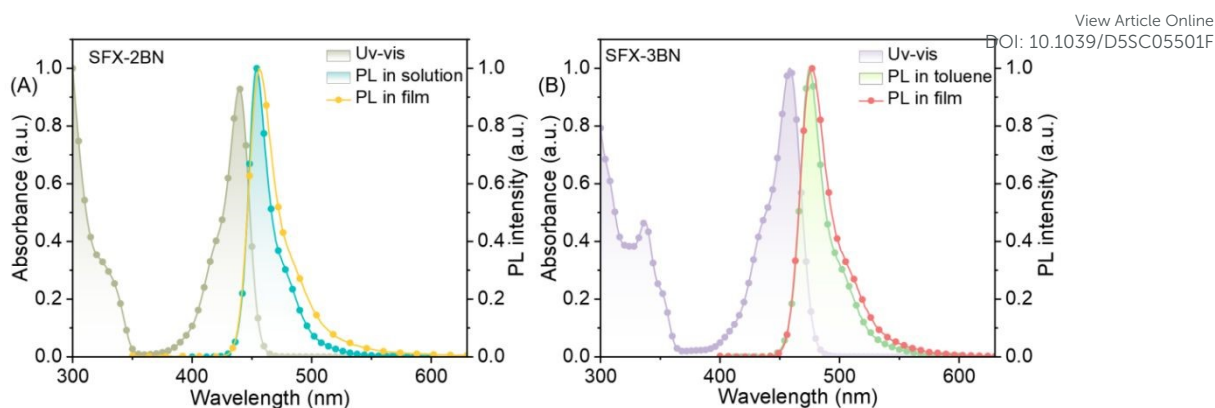
Fig. 4. The UV-Vis absorption and PL spectra in dilute toluene ( 1 \times 10^{-5} M) and mCP-doped films for SFX-2BN (A) and SFX-3BN (B).
