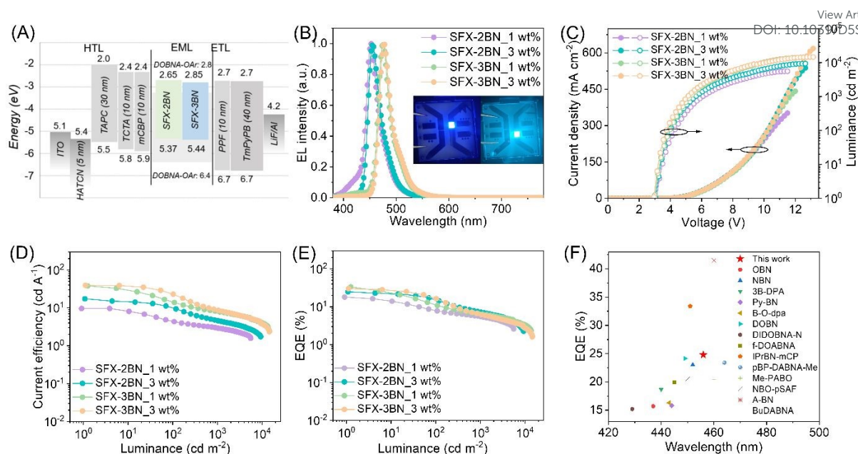
Fig. 5. (A) Schematic diagram of the device configuration, (B) the EL spectra, (C) J-V-L characteristic, (D and E) the efficiency curves of devices A-D, (F) EQE versus wavelength of some representative blue OLEDs reported in the literature with CIE_y \leq 0.1 .
