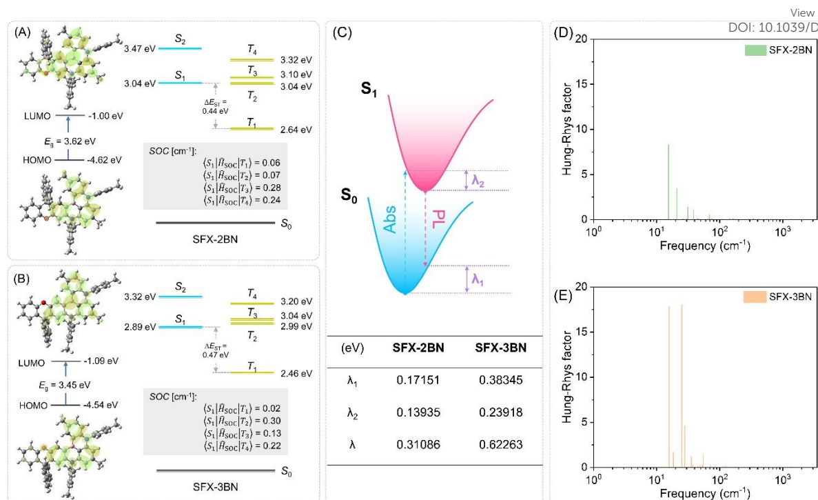
Fig. 3. The calculated FMOs distribution, excited energy levels, SOC values (A and B), the reorganization energy ( \lambda ) (C), and Huang-Rhys (HR) factor (D and E) for the S_1 \rightarrow S_0 transition of SFX-2BN and SFX-3BN, respectively.
