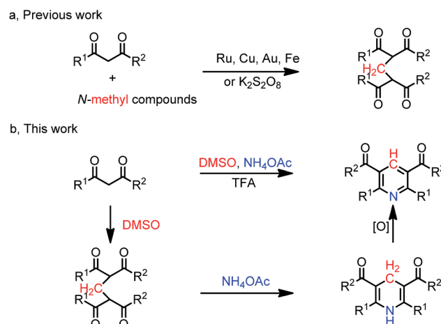
Scheme 1 Methods for the synthesis of methylene-bridged bis-1,3-diketones.
