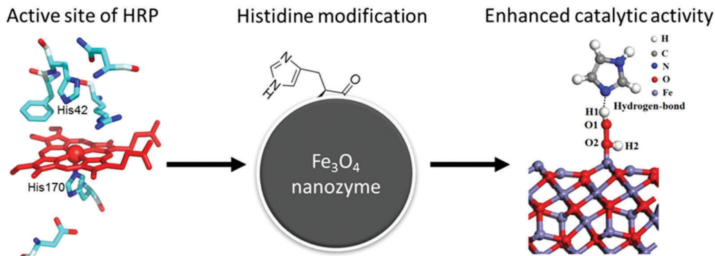
Fig. 24 Mimicking the active site of natural enzymes to improve the peroxidase-like activity of Fe 3 O 4 NPs. Adapted with permission from ref. 724. Copyright (2017) Royal Society of Chemistry.
