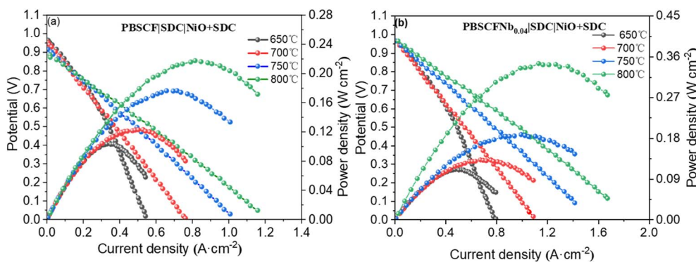
Fig. 8 (a) The power density of a single cell PBSCF|SDC|Ni + SDC at 650–800 °C and (b) the power density of single cell PBSCF 0.04 |SDC|Ni + SDC at 650–800 °C.
