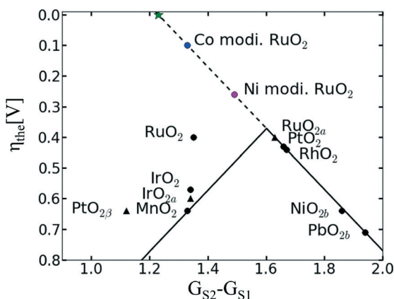
Fig. 8 Updated volcano plot of the one shown in Fig. 5 with the overpotentials of Ni- and Co-modified \text{RuO}_2 . The activation of bridge sites by Ni and Co incorporation into \text{RuO}_2 breaks the scaling relationship between the binding energies of reaction intermediates. The green star marks the position of an ideal catalyst. Reproduced from ref. 76 with permission from the PCCP Owner Societies.
