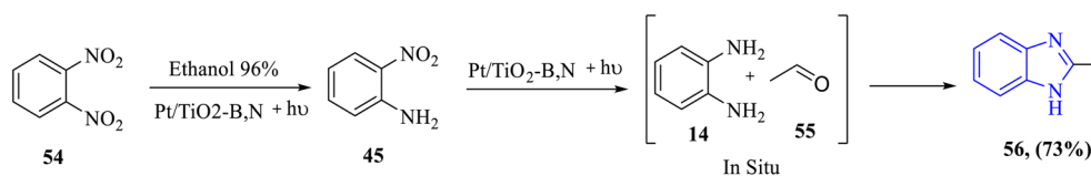
Scheme 15 One-pot synthesis of benzimidazole 56 via photocatalytic reduction of dinitrobenzene ( 54 ) to O -phenylenediamine 14 followed by condensation with aldehyde 55 using a Pt/TiO 2 -B,N catalyst in ethanol.
