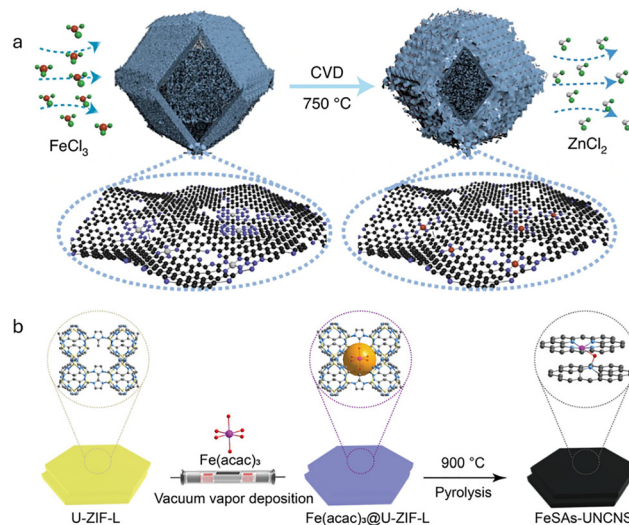
Fig. 4 Schematic CVD synthetic process of Fe–N–C of with (a) FeCl 3 , Reproduce with permission. 50 Copyright © 2021 Springer Nature Limited. (b) Fe(acac) 3 , Reproduce with permission. 51 Copyright © 2024 John Wiley & Sons, Inc or related companies.
