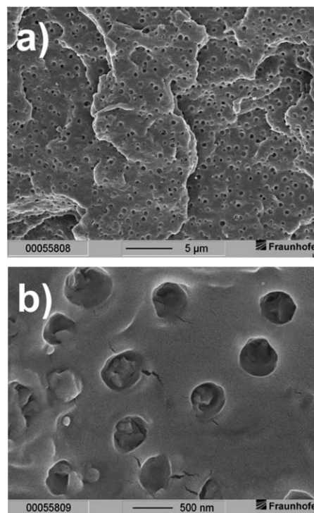
Fig. 4 Scanning electron microscopy pictures of a freeze-fractured surface of PLA composite I at two different magnifications (scaling: (a) 5 \mu m and (b) 500 nm).
