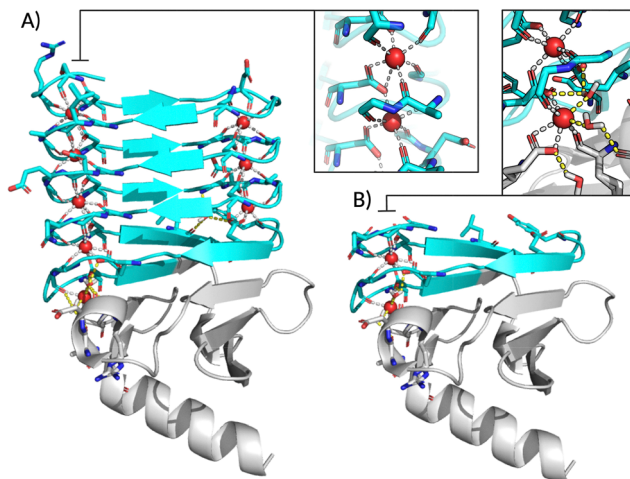
Fig. 1 (A) Crystal structure of block V of the RTX domain, RTX(8), showing eight calcium-bound sites (PDB ID: 5CVW). (B) Truncated scaffold RTX(2), retaining the two C-terminal calcium-binding sites. Inset: Calcium coordination geometries vary across RTX(8), with the RTX(2) region exhibiting a dense, water-mediated second-shell hydrogen-bonding network. Gray dashed lines represent coordination bonds to protein residues, and yellow dashed lines indicate water-mediated coordination and hydrogen bonding interactions.
