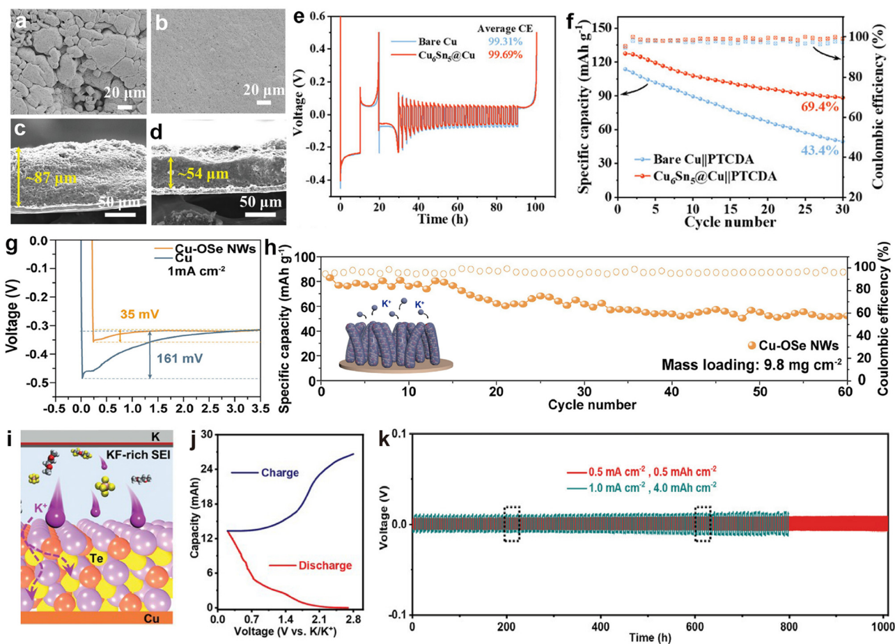
Fig. 17 SEM images of K electroplating on (a) bare Cu and (b) \text{Cu}_6\text{Sn}_5@\text{Cu} . Cross-sectional SEM images of K electroplating on (c) bare Cu and (d) \text{Cu}_6\text{Sn}_5@\text{Cu} with a capacity of 2 \text{ mA h cm}^{-2} . (e) CE of bare Cu and \text{Cu}_6\text{Sn}_5@\text{Cu} current collectors at 1 \text{ mA cm}^{-2} with a capacity of 1 \text{ mA h cm}^{-2} . (f) Cyclic performance of bare \text{Cu}||\text{PTCDA} and \text{Cu}_6\text{Sn}_5@\text{Cu}||\text{PTCDA} anode-free full cells at 20 \text{ mA g}^{-1} . Reproduced with permission from ref. 204. Copyright 2024, Wiley-VCH. (g) Voltage profiles of K nucleation at 1 \text{ mA cm}^{-2} . (h) Cycling performance of the anode-free \text{K}_{0.5}\text{MnO}_2||\text{Cu-OSe NWs} full cell at 100 \text{ mA g}^{-1} . The inset shows a schematic of K deposition behavior on Cu-OSe NWs. Reproduced with permission from ref. 205. Copyright 2024, Elsevier. (i) Cross-sectional schematic diagram displaying the interior configuration of PMBs. (j) Typical charge/discharge profiles at 0.1 \text{ mA cm}^{-2} and -40 \text{ }^\circ\text{C} . (k) Galvanostatic cycling performance of K||K symmetric cells with 0.5 \text{ M KPF}_6/\text{DME-3TTE} . Reproduced with permission from ref. 206. Copyright 2022, Wiley-VCH.
