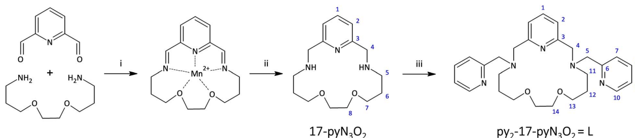
Fig. 2 Synthetic scheme for macrocycles 17-pyN 3 O 2 and L together with the atom numbering used for NMR assignment for both macrocycles; (i) \text{MnCl}_2 \cdot 4\text{H}_2\text{O} , methanol; (ii) \text{NaBH}_4 , \text{O}_2 , \text{H}_2\text{O} ; 73%; (iii) 2-(chloromethyl)pyridine, anhydrous \text{K}_2\text{CO}_3 , anhydrous acetonitrile; 68%.
