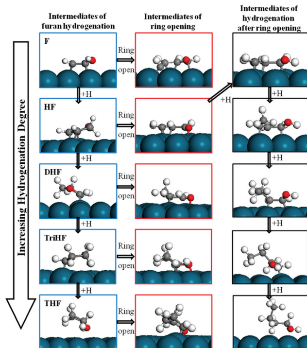
Fig. 14 Structures of intermediates along the pathways of furan hydrogenation (blue), ring opening (red) and hydrogenation (black) after ring opening. The figure shows the intermediates uplifting with increasing degree of hydrogenation.
