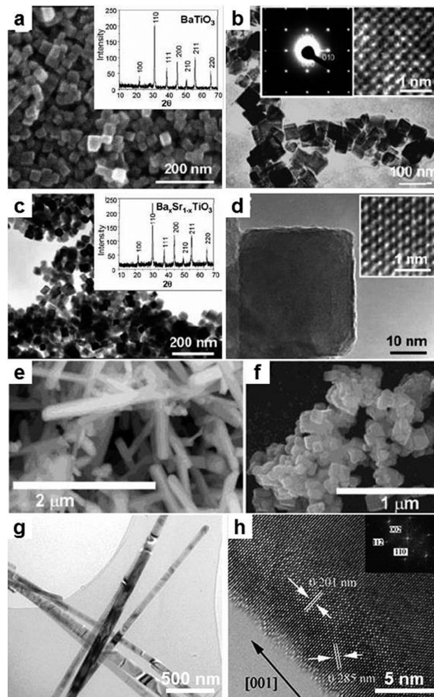
Fig. 7 BaTi(Sr)O_3 nanostructures synthesized in different salt systems. (a–d) BaTiO_3 NCs synthesized in molten NaOH/KOH at 200^\circ C from BaCl_2 and TiO_2 . (a and c) SEM and (b and d) TEM images of BaTiO_3 and BaTi_{1-x}Sr_xO_3 NCs. The insets in (a and c) are XRD patterns, and in (b and d) are HRTEM images. (Reprinted with permission from ref. 76. Copyright 2006 American Chemical Society.) (e) SEM images of BaTiO_3 nanowires and (f) SrTiO_3 nanocubes synthesized in NaCl at 820^\circ C in the presence of surfactant. (Reprinted with permission from ref. 77. Copyright 2003 American Chemical Society.) (g) TEM and (h) HRTEM images of BaTiO_3 nanobelts synthesized in NaCl/KCl at 950^\circ C . (Reproduced from ref. 79 with permission from The Royal Society of Chemistry.)
