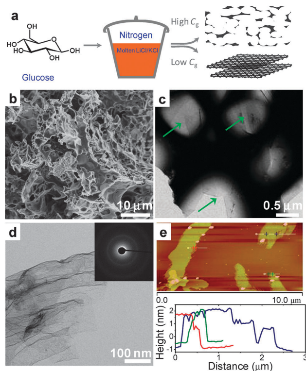
Fig. 23 Graphene from glucose by SMS. (a) Schematic of conversion of glucose to porous carbon (or graphene) at high (or low) glucose concentration (C g ) in LiCl/KCl melt. (b) SEM and (c) TEM images of the porous carbon synthesized at 800 °C with high C g (glucose/salt = 1/10). The green arrows in (c) point the thin-layer at the edge of the main structure. (d) TEM and (e) AFM images for the graphene synthesized from glucose at low C g (glucose/salt = 1/100). (Reprinted with permission from ref. 169. Copyright 2013 John Wiley and Sons.)
