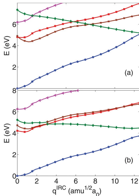
Fig. 8 A' Ground state (blue circles), A'1\pi\pi^* (red squares), A'1\pi\sigma^* (brown crosses), A'2\pi\pi^* (green diamonds) and A'2\pi\sigma^* (magenta triangles) potential energy profiles computed at the SA5-CASSCF (a) and XMCQDPT2 (b) levels of theory along the IRC scan on the A'2\pi\pi^* state.
