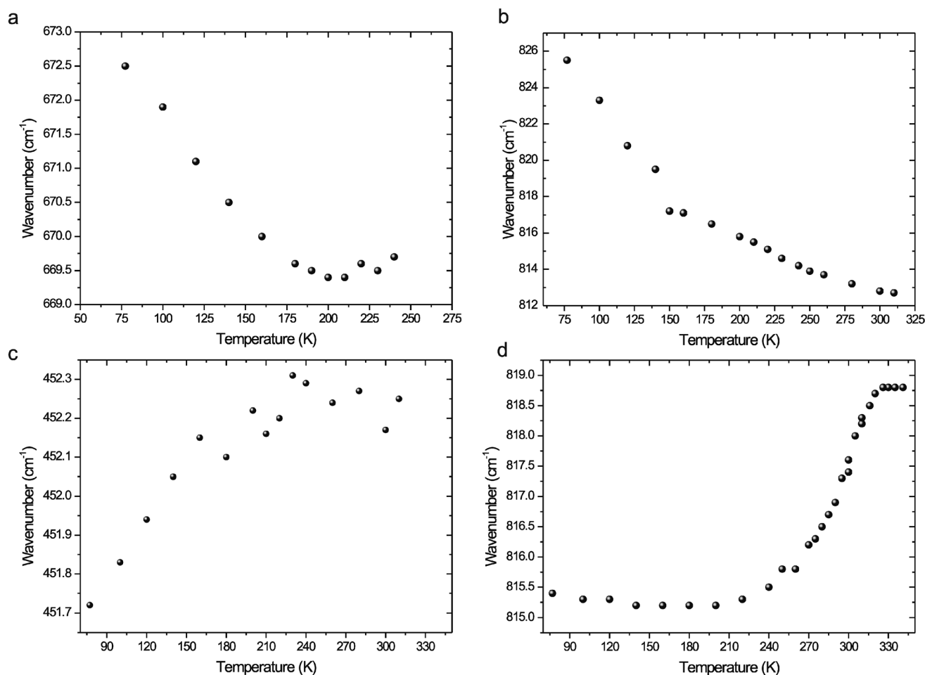
Fig. 10 Temperature dependence of the position of selected bands from FTIR spectra: (a) a band at 669 cm -1 of the 2-athd 2 SeO 4 ·H 2 O spectrum; (b) a band at 813 cm -1 of the 2-athdH 2 SO 4 spectrum; (c) a band at 452 cm -1 of the 2-athdClO 4 spectrum; (d) a band at 818 cm -1 of the 2-athd 2 ClO 4 spectrum. Mentioned band positions were recorded at room temperature.
