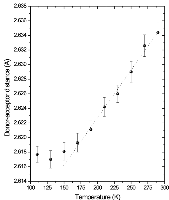
Fig. 11 Temperature dependence of the donor⋯acceptor ( \text{O4}\cdots\text{O3}^\circ ) distance of the O–H⋯O hydrogen bond in 2\text{-athdHSO}_4 . Dashed line represents ideal linear dependence.
