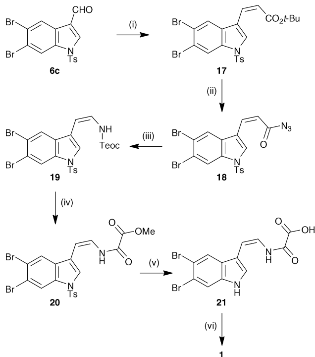
Scheme 3 Total synthesis of kottamide E. Reagents and conditions: (i) t -BuO 2 -CCH 2 P(O)(OPh) 2 , NaH, THF, -78 °C, 78% + 5% ( E )-isomer; (ii) TFA, CH 2 Cl 2 then NaH, DPPA, THF; (iii) TMSCH 2 CH 2 OH, toluene, reflux; (iv) NaHMDS, MeO 2 CC(O)Cl, THF then TBAF, THF, 32% over 5 steps; (v) aq. NaOH, MeOH, THF, 97%; (vi) 3-HCl, HBTU, DMF, Et 3 N, 38%.
