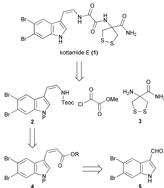
Scheme 1 Retrosynthetic analysis of kottamide E.
