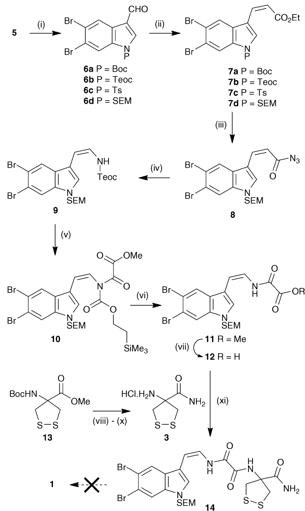
Scheme 2 Synthesis of SEM-protected kottamide E. Reagents and conditions: (i) for 6a : NaH, di- tert -butyl dicarbonate, THF, 95%; for 6b : NaH, 4-nitrophenyl 2-(trimethylsilyl)ethyl carbonate, THF, 95%; for 6c : NaH, TsCl, THF, 81%; for 6d : NaH, SEMCl, THF, 95%; (ii) EtO 2 CCH 2 P(O)(OPh) 2 , NaH, THF, -40 °C. For 7a : 81% + 13% ( E )-isomer; for 7b : 81% + 13% ( E )-isomer; for 7c : 80%; for 7d : 68% + 31% ( E )-isomer 15 ; (iii) aq. NaOH, MeOH, THF, 65 °C then NaH, DPPA, THF, 91%; (iv) TMSCH 2 CH 2 OH, toluene, reflux, 77%; (v) NaHMDS, MeO 2 CC(O)Cl, THF, 0 °C; (vi) TBAF, THF, 0 °C, 66% over 2 steps; (vii) aq. NaOH, MeOH, THF, 100%; (viii) aq. NaOH, THF, MeOH, 99%; (ix) i -BuOC(O)Cl, Et 3 N, THF, 0 °C then NH 3 , MeOH, -20 °C, 89%; (x) SOCl 2 , MeOH, 50 °C, 100%; (xi) HBTU, DMF, Et 3 N, 50 °C, 66%.
