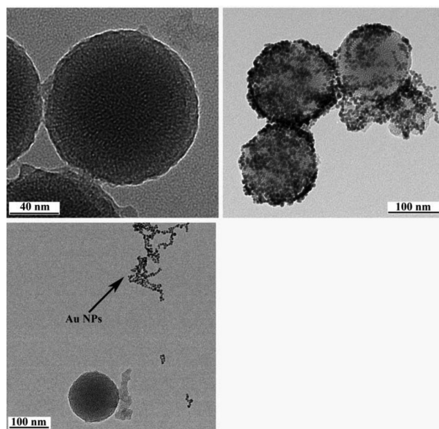
Fig. 1 Transmission electron micrographs of bare MSN (a), AuNPs-capped-MSN at pH 5 (b) and pH 4 (c) after 20 h. Arrow indicates aggregated gold nanoparticles. Samples were obtained by dropping 5 \mu\text{L} of PBS solution with different pH containing 0.1 mg mL -1 AuNPs-capped-MSN or MSN onto carbon-coated copper grids, and then dried for 10 h in air.
