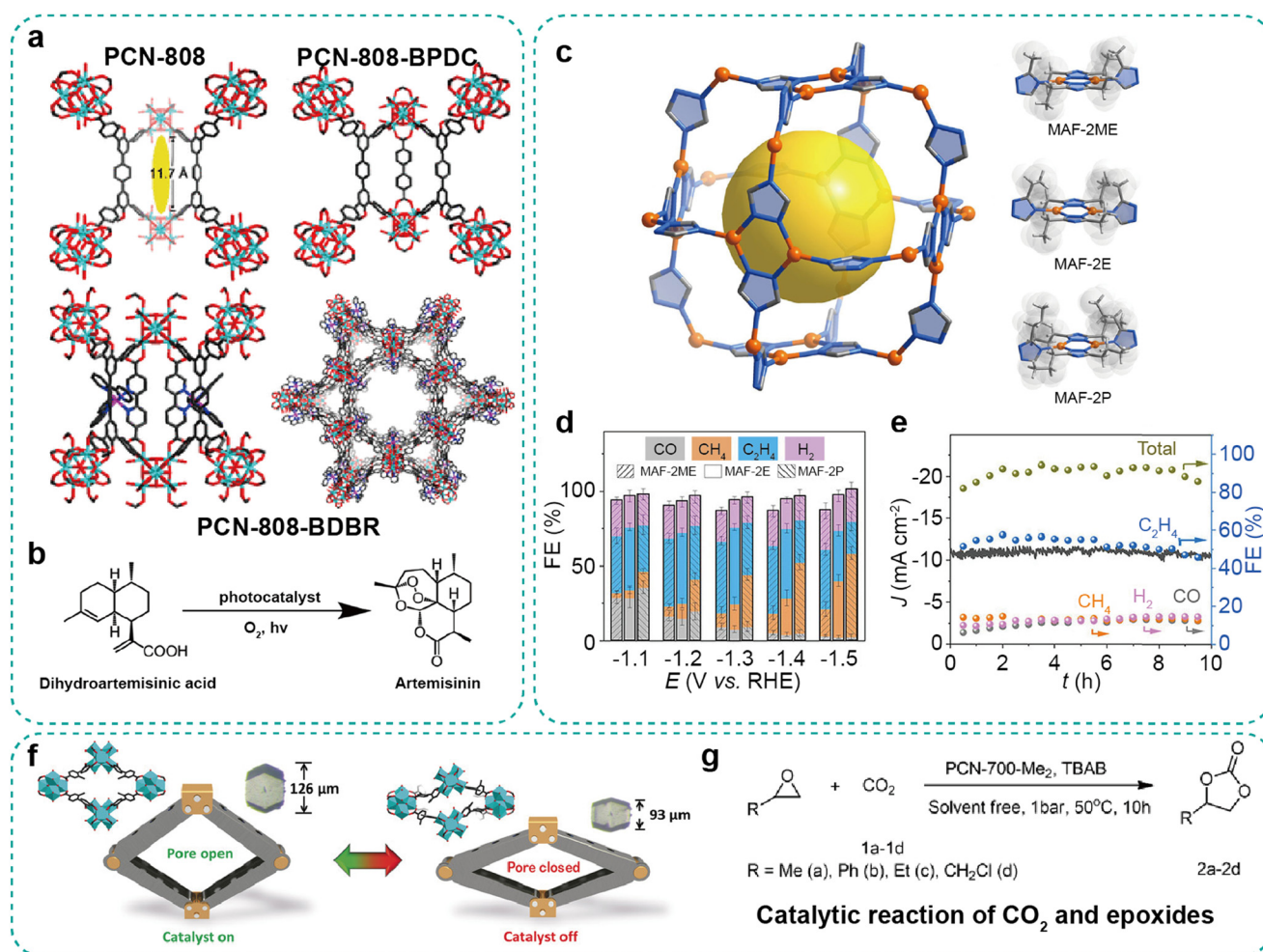
Fig. 6 Soft MOFs for catalysis. (a) Crystal structures of PCN-808 series; (b) photocatalytic oxidation of dihydroartemisinin acid to artemisinin. Reproduced with permission. 60 Copyright 2020, American Chemical Society. (c) Crystal structures of MAF-2 analogs and the corresponding local coordination environments; (d) potential-dependent faradic efficiency of gas products; (e) long term stability of MAF-2 analogs by chronoamperometry. Reproduced with permission. 61 Copyright 2022, Wiley-VCH. (f) Schematic representation of PCN-700-Me 2 before and after desolvation; (g) catalytic reaction of CO_2 and epoxides. Reproduced with permission. 62 Copyright 2016, Wiley-VCH.
