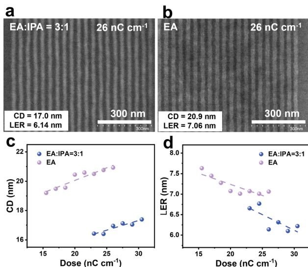
Fig. 3 SEM images of lines with a period of 40 nm at 26 nC cm -1 dose for thinner Sn4-MB films developed using (a) EA:IPA = 3:1 and (b) EA; relation of 40 nm pitch line (c) CD and (d) LER with dose after EA:IPA = 3:1 and EA development of thinner Sn4-MB films upon EBL line-exposure.
