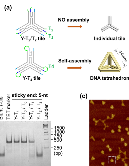
Fig. 2 Assembly of a TET from Y-tiles with cleaved and intact control loops. (a) Schematic diagram of the assembly of Y-T 2 /T 2 and Y-T 4 tiles. The length of each edge of the TET was four turns (42 base-pairings). (b) 3% native PAGE analysis of the self-assembly products of Y-T 2 /T 2 and Y-T 4 tiles with a 5-nt sticky end. (c) Atomic force microscopy (AFM) image of the assembly products of the Y-T 4 tile. The inset shows a close-up view of the particle marked with a white square. The scale bar in the inset is 15 nm.
