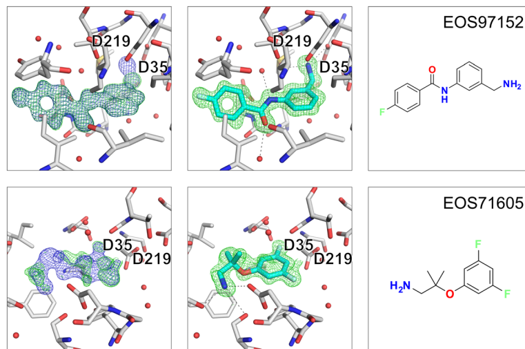
Fig. 5 Two follow-up compounds were found by X-ray crystallography. Close-up of crystallographic follow-up hits. The three panels from left to right show first the (2mF_o-DF_c, \alpha_c) maps contoured at \sigma = 1 (blue) and the (mF_o-DF_c, \alpha_c) maps contoured at \sigma = 3 (green) after auto-refinement with fspipeline, the second panel the omit-map around the ligand after refinement with the ligand placed in green and last the chemical structure of the fragment hit. The catalytic residues Asp35 and Asp219 are annotated.
