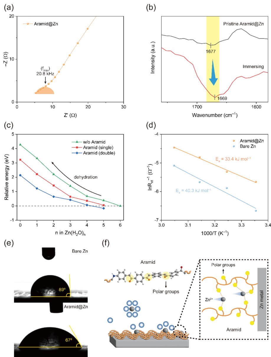
Fig. 3 (a) Enlarged EIS plot of Aramid@Zn symmetric cells. (b) FT-IR spectra of the aramid layer with/without immersing in 2 M \text{ZnSO}_4 electrolyte for 24 h. The spectra were shown in the range of 1600\text{--}1700\text{ cm}^{-1} to indicate the variation of \text{C}=\text{O} . (c) Relative energy of hydrated \text{Zn}(\text{H}_2\text{O})_n complex with and without aramid chains in reference to the fully hydrated state ( n = 6 ). (d) The activation energy of Bare Zn and Aramid@Zn anodes. (e) Contact angles of 2 M \text{ZnSO}_4 electrolyte on the Bare Zn and Aramid@Zn anodes. (f) Schematic illustration of ion-transport process in aramid polymer coating.
