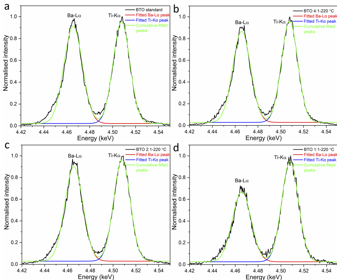
Fig. 8 Fit of the WDS spectra peaks for the Ba- L_{\alpha} and Ti- K_{\alpha} peaks of (a) the standard \text{BaTiO}_3 and \text{BaTiO}_3 samples hydrothermally synthesised at 220 °C using Ba/Ti precursor ratios of (b) 4 : 1, (c) 2 : 1 and (d) 1 : 1 (sample labels explained in Table 1).
