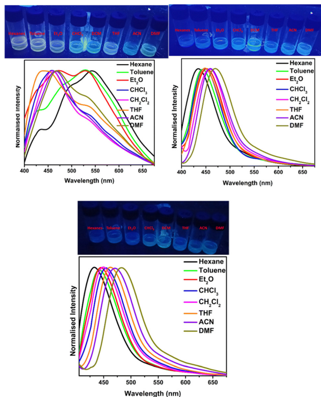
Fig. 31 The FI spectra of compound 43a (top left), 43b (top right) and 43c (bottom) at various solvents; inset: digital photos taken under 365 nm UV light. Reproduced with permission from ref. 42. Copyright 2023 Royal Society of Chemistry.
