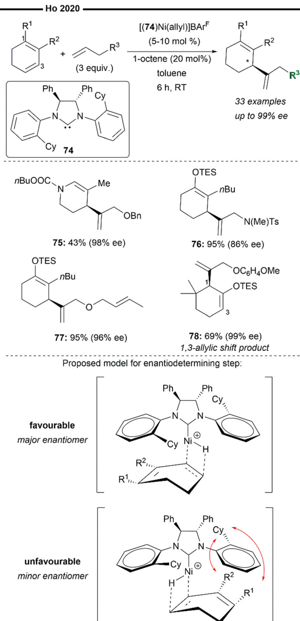
Scheme 15 Ni/chiral NHC catalysed enantioselective synthesis of 1,4-dienes by cross-hydroalkenylation of endocyclic 1,3-dienes and hetero-substituted terminal alkenes. 66
