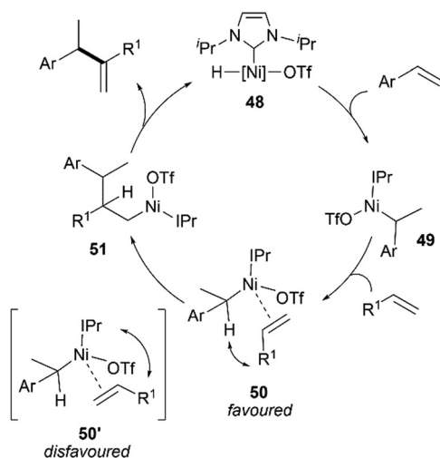
Scheme 10 Ni/NHC catalysed branched-selective hetero-hydroalkenylation of styrenes and unactivated \alpha -olefins. 60
