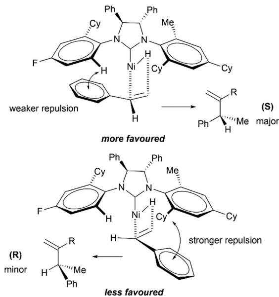
Scheme 11 Asymmetric Ni/chiral NHC catalysed hetero-hydroalkenylation of styrenes and \alpha -olefins. 61
