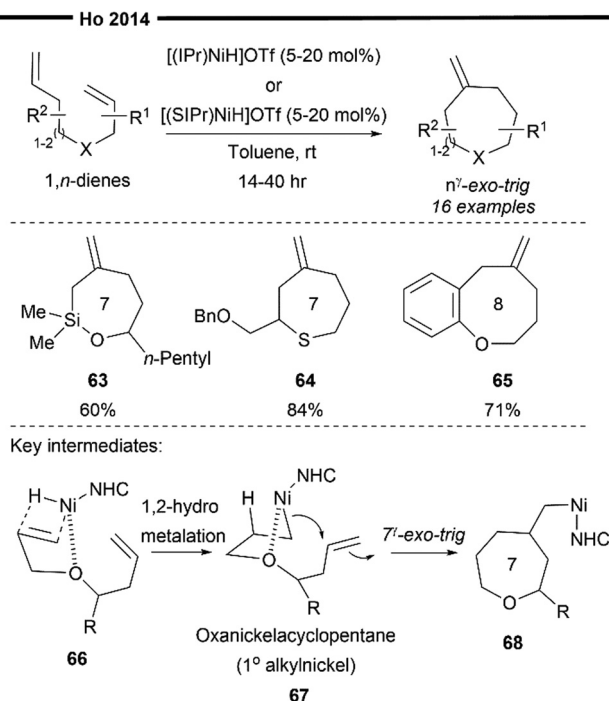
Scheme 13 Ni/NHC catalysed cycloisomerisation of 1, n -dienes. 63
