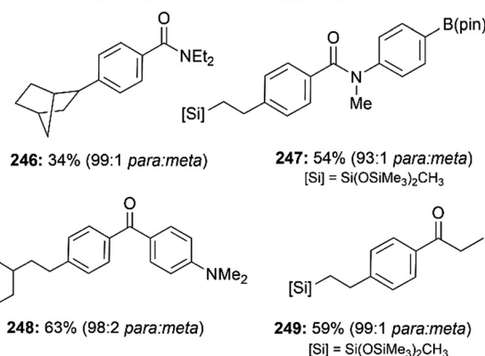
Scheme 40 NHC–Ni/Al catalysed para -selective C–H alkylation of benzamides and aromatic ketones via hydroarylation with alkenes. 104
