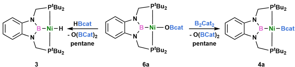
Scheme 3 Reactivity of t BuPBPNIH 2 Bcat ( 6a ) with B 2 Cat 2 to form 4a (right) and with HBcat to form 3 (left).
