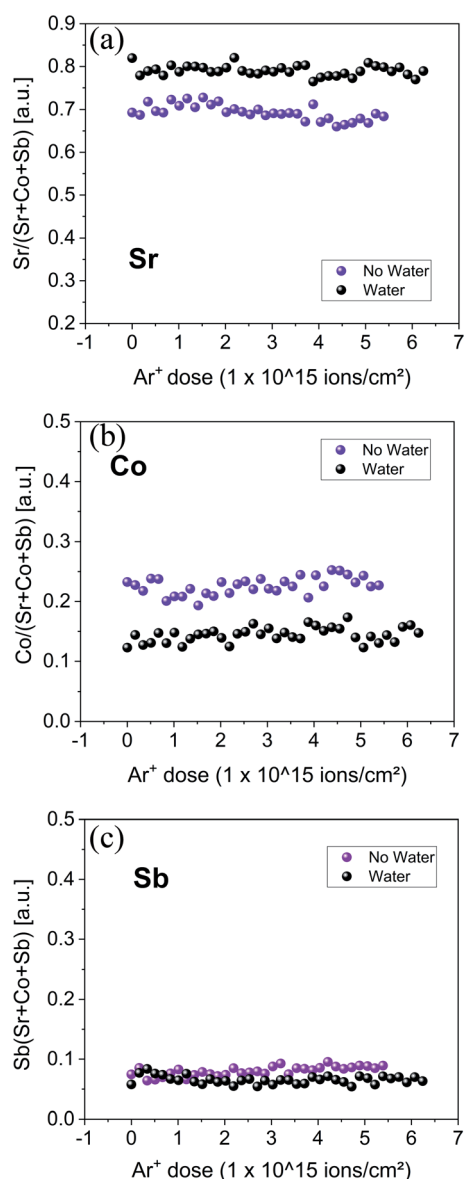
Fig. 1 \text{Ne}^+ 5 keV depth profile LEIS analysis of SCS powders. For each spectrum, the Sr, Co and Sb species energy peaks were integrated, and the intensities plotted as a function of the total \text{Ar}^+ sputtering dose. The as-synthesized powder (purple dots) and the same batch of powder but analyzed after being dipped in water and dried at 100 °C (black dots) are compared.
