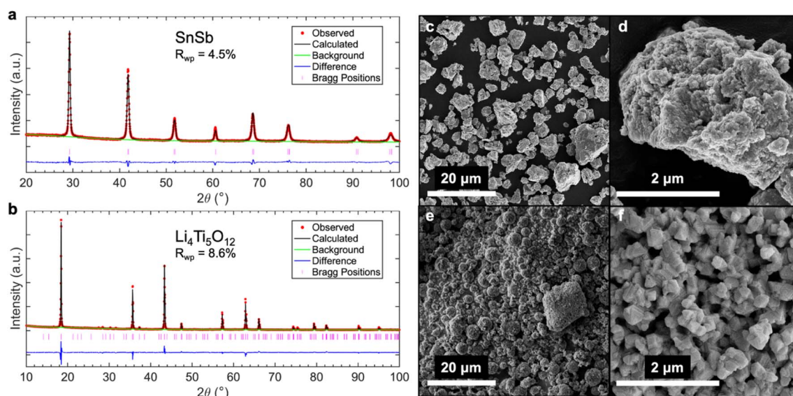
Fig. 2 Rietveld-refined X-ray diffraction patterns of (a) SnSb and (b) \text{Li}_4\text{Ti}_5\text{O}_{12} (LTO) revealing profile residual ( R_{\text{wp}} ) factors < 10%, indicating phase-pure materials. Scanning electron micrographs (SEM) of (c and d) SnSb particles and (e and f) \text{Li}_4\text{Ti}_5\text{O}_{12} particles at both low- and high-magnification, respectively.
