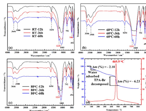
Fig. 4 FTIR spectra of ZSM-5 after various gel aging conditions: RT (a); 60 °C (b); and 80 °C (c). TGA-DSC curve (d) of ZSM-5 zeolites.
