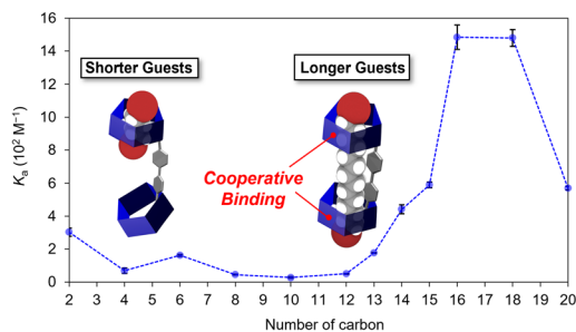
Fig. 4 Plot of the association constants ( K_a ) for BPh (1.0 mM, \text{CDCl}_3 , 295 K) with \alpha,\omega -dibromoalkanes ( \text{C}_n , n = 2, 4, 6, 8, 10, 12-16, 18 , and 20). The illustrations depict 1 : 1 host–guest complexes of BPh with C2 and C14, as suggested by Job's plots.
