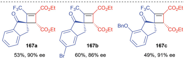
Scheme 47 Michael addition/Wittig olefination reaction of CF_3 -substituted spirocyclobutene.
