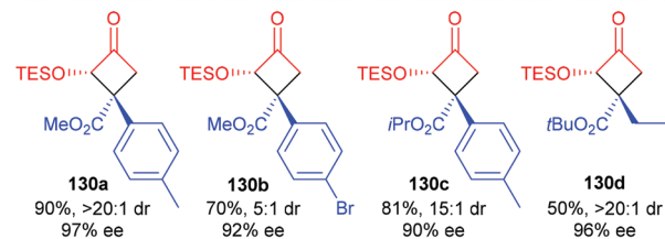
Scheme 37 Tandem cyclopropanation/semipinacol rearrangement.
