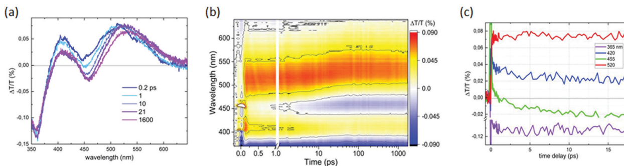
Fig. 3 \Delta T/T spectra of C-dots produced by the space-confined vacuum-heating approach: (a) spectra for selected time delays, (b) map, (c) dynamics for selected wavelengths; pump@400 nm with fluence of 6.5 \text{ mJ cm}^{-2} , pump and probe polarization are set at magic angle.
