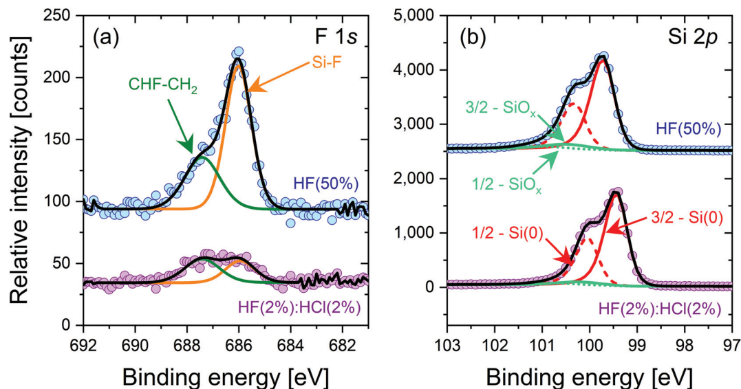
Fig. 4 XPS spectra at take-off angle of 15° with respect to the surface parallel for 5 Ω cm n-type FZ-Si treated for 10 min with HF(50%) at the top, and HF(2%) : HCl(2%) at the bottom. Spectra have been offset in the vertical direction for clarity. The F 1s spectra (left) show substantially enhanced fluorine termination in the HF(50%) case. The Si 2p spectra (right) are similar for both treatments, showing any SiO x layer is thin. Additional superacid-derived passivation was not applied.
