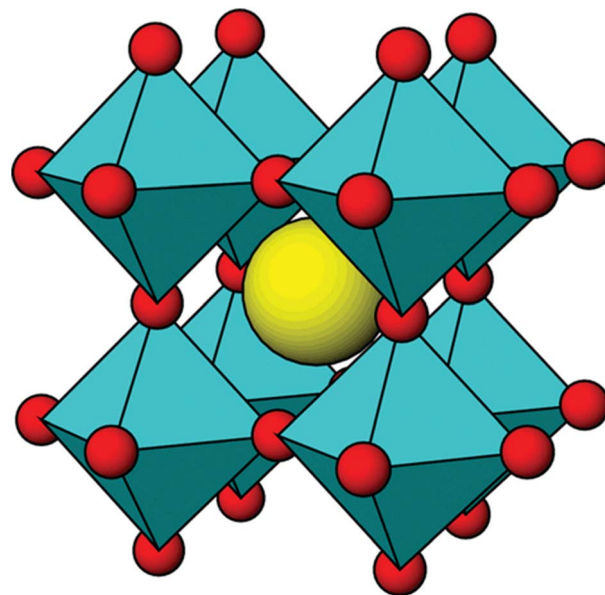
Fig. 1 Ideal cubic perovskite structure for ABO_3 ( BO_6 units – cyan; A atoms – yellow; O atoms – red). 38 This figure has been reproduced from ref. 38 with permission from Frontiers in Chemistry , copyright 2025.
