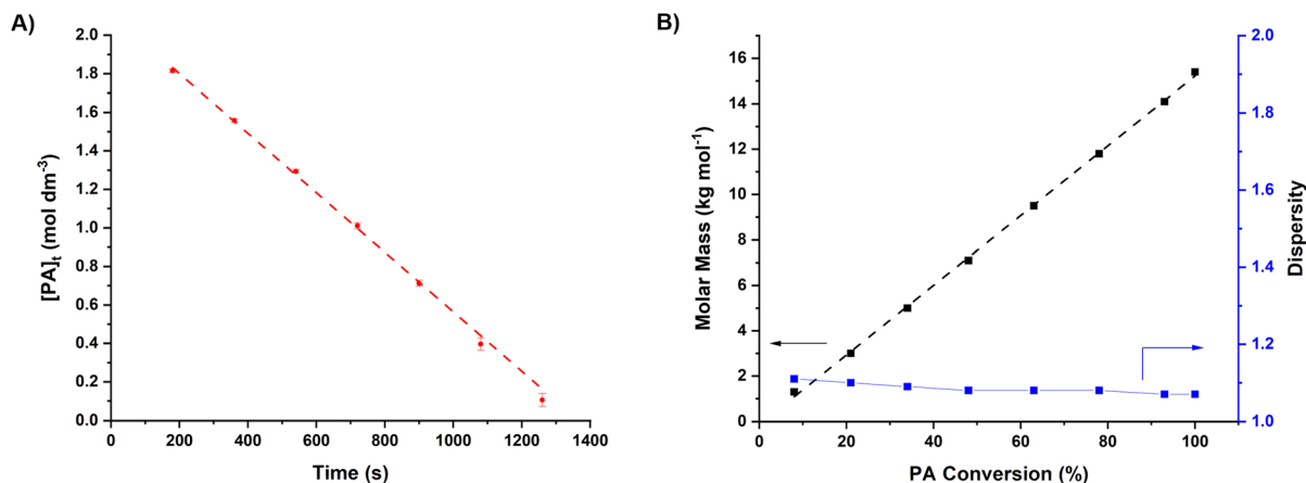
Fig. 2 Catalyst benchmark data for the ROCOP of CHO and PA with complex 2 . Conditions: [2] : [PA] : [CHO] = 1 : 400 : 2000 , T = 100 °C. (A) Plot of [PA]_t vs. time (s). Reaction displays a zero-order dependence on [PA]_t . Reactions repeated in triplicate, with average values of [PA]_t plotted. (B) Plot of polymer molar mass, and dispersity, against PA conversion.
