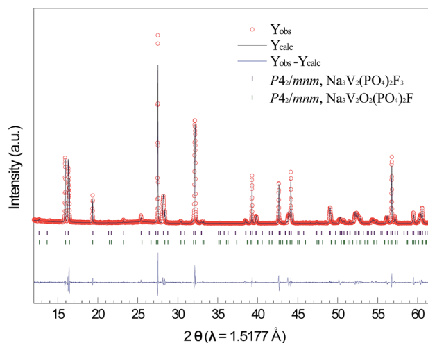
Fig. 2 Synchrotron XRD data and whole pattern fitting of the NVOPF-rGO composite.
