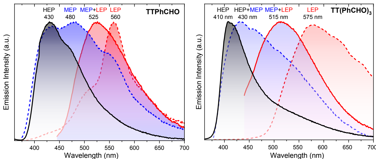
Figure 4. Normalized PL and Phosphorescence spectra of crystals of TTPhCHO (left) and TT(PhCHO) 3 (right) at 298 K. Left: prompt (full lines: black, \lambda_{\text{exc}} = 340 nm; red, \lambda_{\text{exc}} = 430 nm) and delayed emissions (dashed \lambda_{\text{exc}} = 300 nm: blue, delay 20 \mu s, window 0.1 ms; red, delay 50 \mu s, window 0.5 ms). Right: prompt (full lines: black, \lambda_{\text{exc}} = 340 nm; red, \lambda_{\text{exc}} = 420 nm) and delayed emissions ( \lambda_{\text{exc}} = 340 nm, blue, delay 20 \mu s, window 200 \mu s; red, delay 100 \mu s, window 1 ms).
