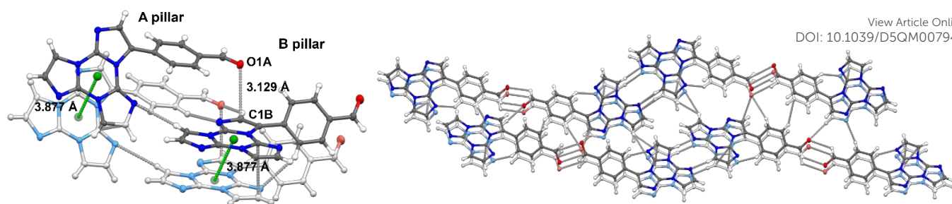
Figure 7. Fragments of crystal packing of TTPhCHO highlighting (left) the stacked motif of A and B molecules, with triazinic centroids plotted as green spheres, and the close carbonyl...TT contact, and (right) two overlapped pairs of HB- and C=O...C=O bonded chains. Intermolecular contacts shorter than the sum of vdW radii are plotted with dashed grey lines. Ellipsoids are drawn at the 20% probability level.
