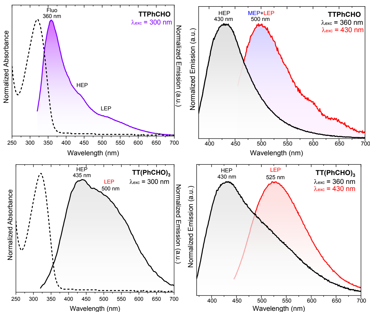
Figure 2. Normalized Spectra of PMMA film (0.5 w/w%) of TTPhCHO (upper panel) and TT(PhCHO) 3 (bottom panel) at 298 K. Left: Absorption (dash lines) and PL emission (full lines, \lambda_{\text{exc}} = 300 nm). Right: PL emission at \lambda_{\text{exc}} = 360 (black lines) and 430 nm (red lines).
