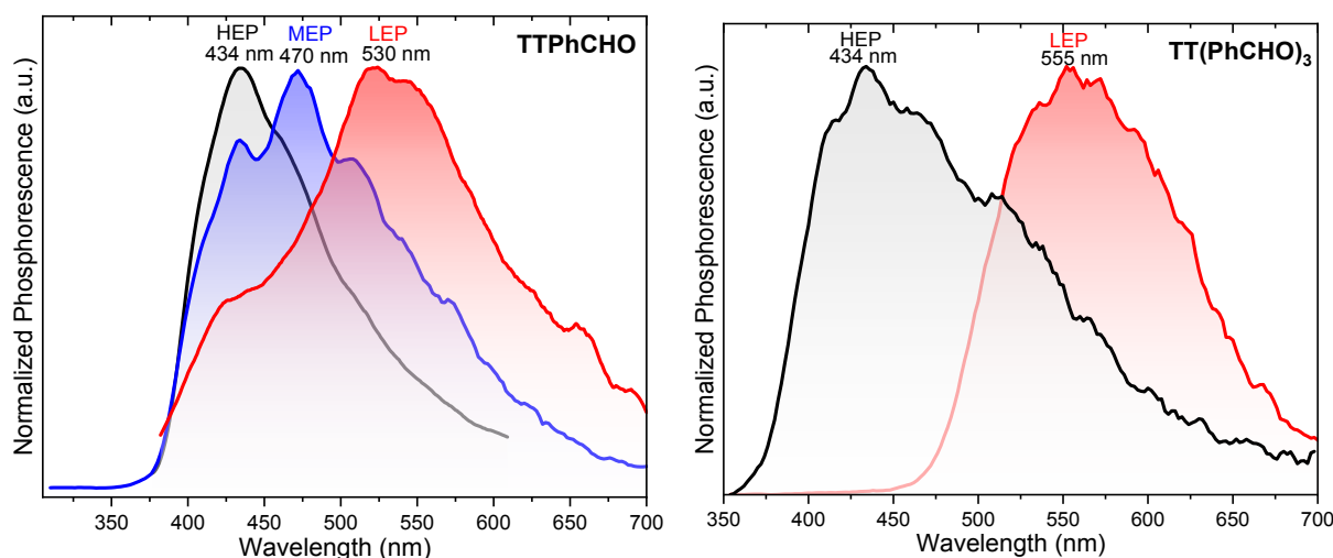
Figure 3. Normalized Phosphorescence spectra at 298 K of PMMA film (0.5 w/w%) of TTPhCHO (left: black line, \lambda_{\text{exc}} = 250 nm, delay 50 \mu\text{s} , window 0.5 ms; blue line, \lambda_{\text{exc}} = 280 nm, delay 0.2 ms, window 0.5 ms; red line, \lambda_{\text{exc}} = 300 nm, delay 0.1 ms, window 5 ms) and TT(PhCHO) 3 (right: red line, \lambda_{\text{exc}} = 330 nm, delay 0.2 ms, window 0.5 ms; black line, \lambda_{\text{exc}} = 250 nm, delay 1 ms, window 5 ms).
