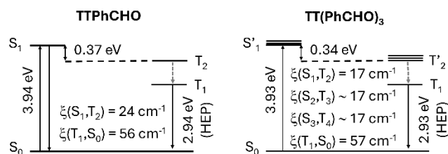
Figure 6. Computed energy diagram and Spin Orbit Coupling matrix elements ( \xi ) for TTPhCHO (left) and TT(PhCHO) 3 (right).
