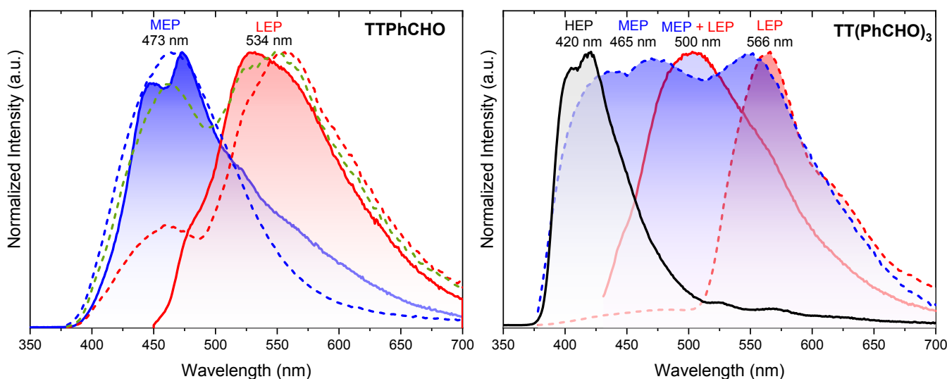
Figure 5. Normalized PL (77 K) and Phosphorescence (87 K) spectra of crystals of TTPhCHO (left) and TT(PhCHO) 3 (right). Left: prompt (full lines: blue, \lambda_{\text{exc}} = 300 nm; red, \lambda_{\text{exc}} = 430 nm) and delayed emissions (dashed lines, \lambda_{\text{exc}} = 300 nm: blue, delay 20 \mu s window 100 \mu s; green, delay 500 \mu s window 2 ms, red, delay 2 ms window 2 ms). Right: prompt (full lines black, \lambda_{\text{exc}} = 300 nm; red, \lambda_{\text{exc}} = 420 nm) and delayed emissions (dashed lines, \lambda_{\text{exc}} = 340 nm: blue, delay 20 \mu s, window 200 \mu s; red, delay 200 \mu s, window 2 ms)
