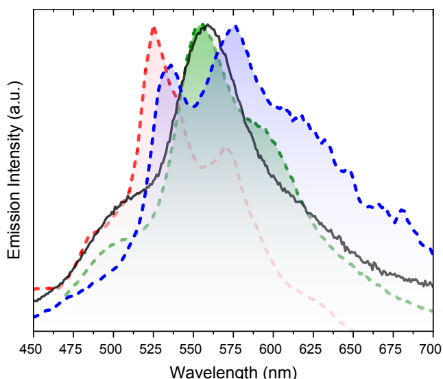
Figure 9. Normalized emission spectra of crystals at 298 K: TTPhCHO (black line: delayed emission, \lambda_{\text{exc}} = 300 nm, delay 50 \mu\text{s} , window 0.5 ms), [Zn 3 (CH 3 COO) 6 (H 2 O) 2 ](TT) 2 (green dashed line: PL at \lambda_{\text{exc}} = 450 nm), TT (red dashed line: delayed emission, \lambda_{\text{exc}} = 374 nm, delay 400 ms, window 1 s) and TT-2pyH (blue dashed line: delayed emission, \lambda_{\text{exc}} = 320 nm, delay 1 ms, window 10 ms)
