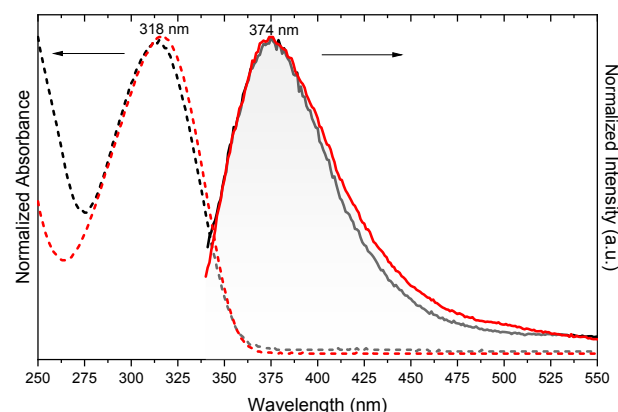
Figure 1. Normalized absorption (dashed lines) and emission (full lines, \lambda_{exc} = 300 nm) of DCM ( 1 \cdot 10^{-5} M) solution of TTPhCHO (black) and TT(PhCHO) 3 (red).
