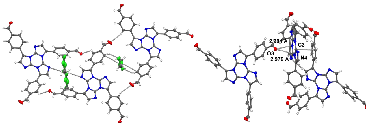
Figure 8. Fragments of crystal packing of TT(PhCHO) 3 highlighting (left) the HB-bonded units hosting the cocrystallized DCM molecules and (right) the close carbonyl...TT contact and the stacked TT...phenyl motif. Intermolecular contacts shorter than the sum of vdW radii are plotted with dashed grey lines. Ellipsoids are drawn at the 20% probability level (only the main component, A, of the disordered molecule is represented).
