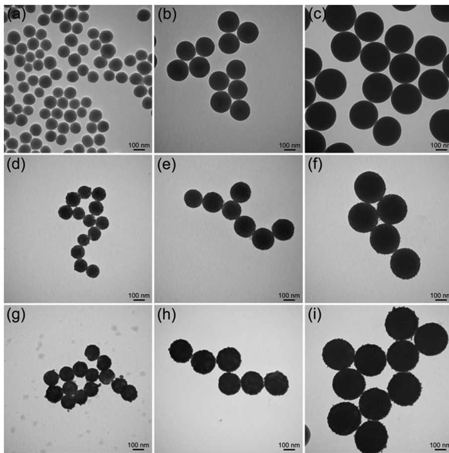
Fig. 5 (a–c) TEM images of \text{SiO}_2\text{@PEI} NPs with different sizes: (a) 120, (b) 200, and (c) 300 nm, and their corresponding fabricated \text{SiO}_2\text{@PEI-Au} seed (d), (e), and (f), and \text{SiO}_2\text{@PEI@Ag} NPs in (g), (h), and (i), respectively.
