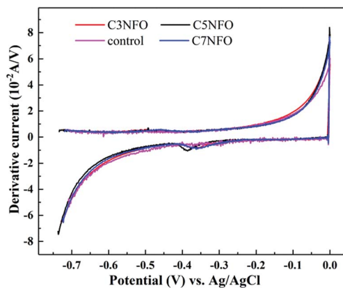
Fig. 6 First derivative of cyclic voltammetry in MFCs with different \text{NiFe}_2\text{O}_4 contents.
