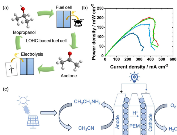
Fig. 9 (a) Schematic of IPA-based LOHC fuel cell system. (b) Power density curves of the IPA-based LOHC fuel cell under 85 °C and varying pressure conditions (100–400 kPa absolute). Reproduced with permission from ref. 60. Copyright 2020, Elsevier. (c) Diagram of ethylamine-based LOHC regenerative fuel cells strategy for emission-free electrical energy storage and generating system.
