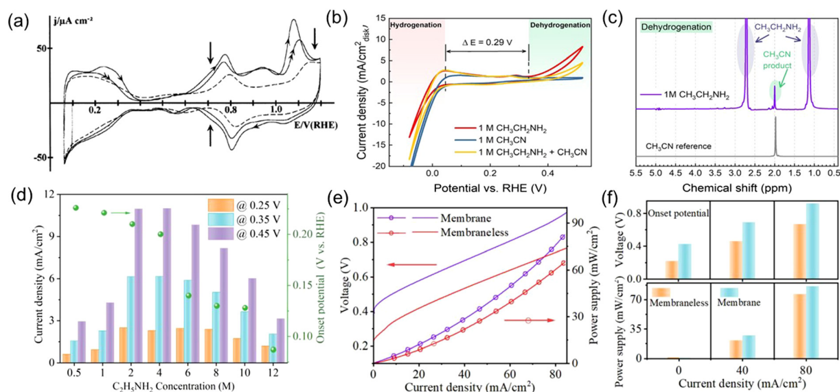
Fig. 5 (a) CV curve for a Pt(111) electrode immersed in 0.1 M HClO 4 + 0.1 M CH 3 CH 2 NH 2 solution. Reproduced with permission from ref. 50. Copyright 1999, Elsevier. (b) CV of commercial Pt black catalyst-loaded working electrode in 1 M NaOH with the addition of 1 M CH 3 CH 2 NH 2 , 1 M CH 3 CN, and 1 M CH 3 CH 2 NH 2 + 1 M CH 3 CN. (c) 1 H NMR spectrum of the liquid product from CH 3 CH 2 NH 2 dehydrogenation obtained by applying 0.7 V vs. RHE for 10 h. Reproduced with permission from ref. 22. Copyright 2021 American Chemical Society. (d) The influences of ethylamine concentration on the EDH onset potential and current density. (e) Polarization curves and power supply profiles using AEM and membraneless ethylamine electrolysis cells. (f) Performance comparison of the two cells regarding cell onset voltage and needed power supply at different current density. Reproduced with permission from ref. 21. Copyright 2023, Elsevier.
