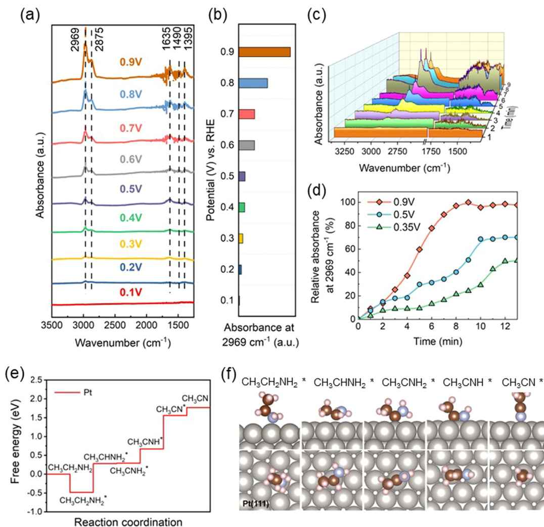
Fig. 4 (a) ATR-IR spectra on Pt in 1 M \text{CH}_3\text{CH}_2\text{NH}_2 + 1\text{ M KOH} solution at various potentials from 0.1 V to 0.9 V vs. RHE. (b) The absorbance on Pt surface at 2969\text{ cm}^{-1} and various potentials from 0.1 V to 0.9 V vs. RHE. (c) Time resolved ATR-IR spectra of Pt surface at 0.9 V vs. RHE. (d) Relative absorbance of pure Pt at 2969\text{ cm}^{-1} at 0.35 V, 0.5 V, and 0.9 V vs. RHE with respect to time. (e) Calculated free energy diagram for EDH. (f) Adsorption configurations of intermediates at Pt surface.
