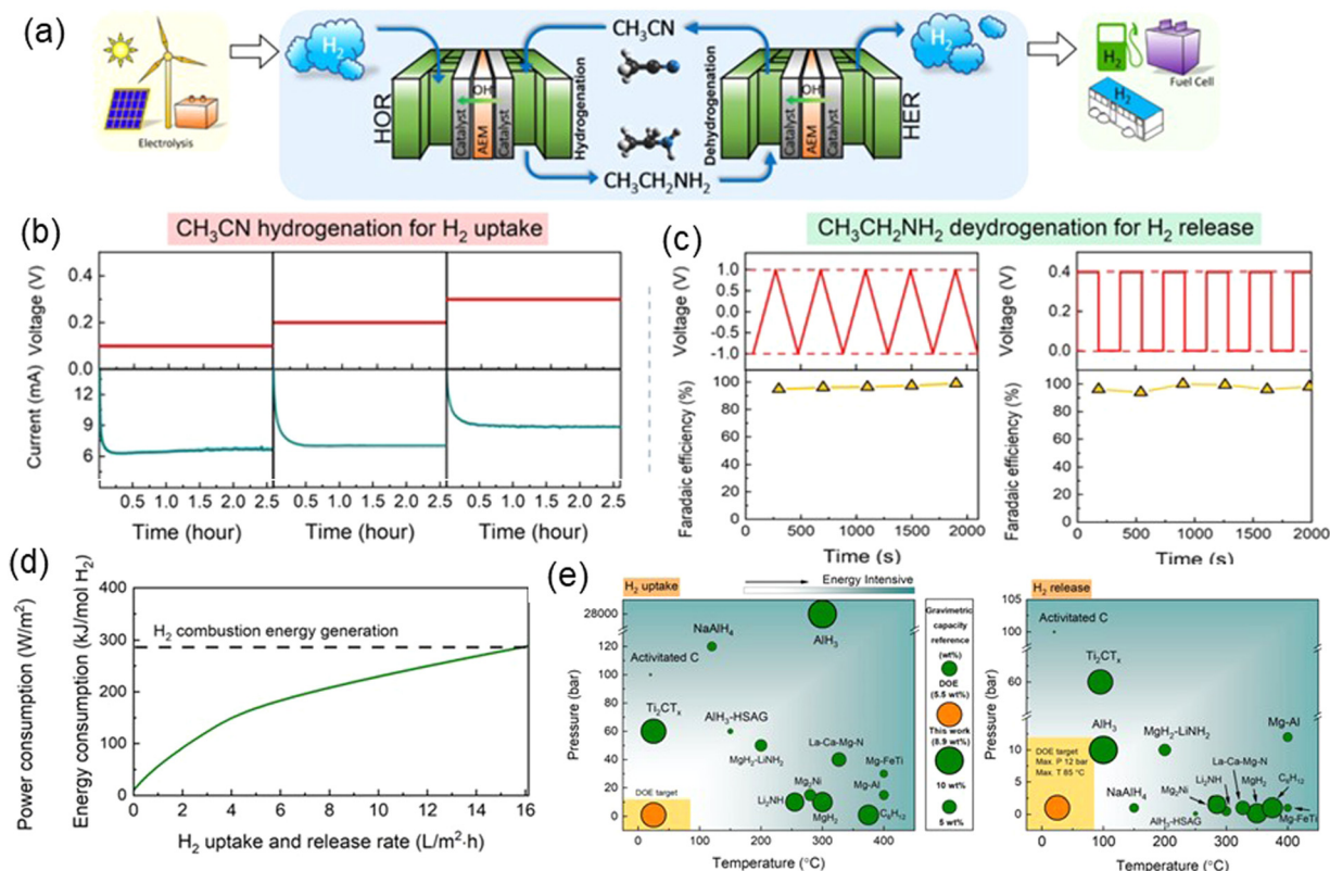
Fig. 8 (a) A blueprint based on ethylamine/acetonitrile that realizes a complete cycle of H 2 production, storage and application under ambient conditions. (b) Hydrogenation of acetonitrile for H 2 uptake under various cell voltages and the measured ethylamine generation rate. (c) Chronoamperometry test of ethylamine dehydrogenation for H 2 release, and the measured H 2 generation FE. (d) Calculated energy consumption for completing a complete H 2 storage cycle as a function of H 2 uptake and release rate. (e) Comparison of the electrochemical ethylamine/acetonitrile redox method with other reported methods in terms of H 2 storage capacity, operation pressure, and temperature. Reproduced with permission from ref. 22. Copyright 2021 American Chemical Society.
