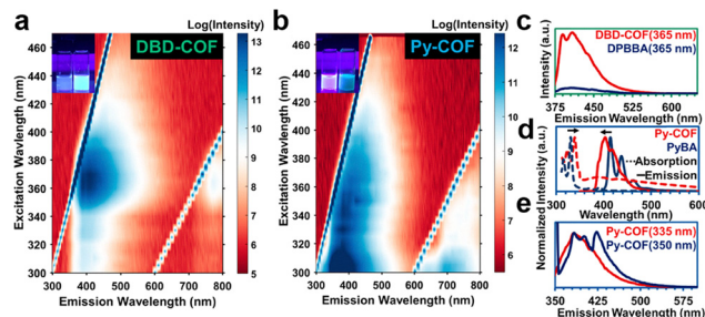
Fig. 64 (a) EEMS of DBD-COF. (Inset) Optical image of the DBPBA monomer (left) and DBD-COF (right) under UV irradiation. (b) EEMS of Py-COF. (Inset) Optical image of the PyBA monomer (left) and Py-COF (right) under UV irradiation. (c) Emission of DBD-COF compared to the DPBBA monomer at the same concentration. (d) Normalized absorption and emission intensity of Py-COF compared to the PyBA monomer showing a red shift of the absorption spectra and blue shift and broadening of the emission spectra. (e) Normalized emission of Py-COF under two excitation wavelengths showing the emergence of an excimer emission (430 nm). Reprinted with permission from ref. 177. Copyright 2019 American Chemical Society.
