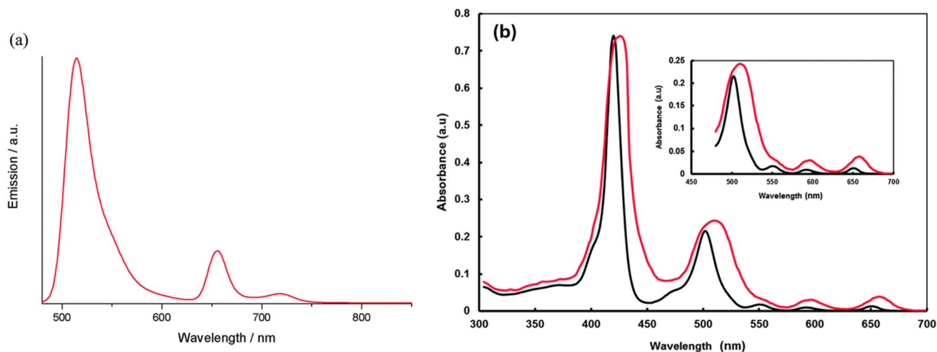
Fig. 19 (a) Emission spectra of conjugate 42 ; (b) normalized absorption spectra of conjugate 42 in THF solution displayed in black line and adsorbed onto TiO 2 film displayed in red line. Reproduced with permission from ref. 89. Copyright 2015, Royal Society of Chemistry.
