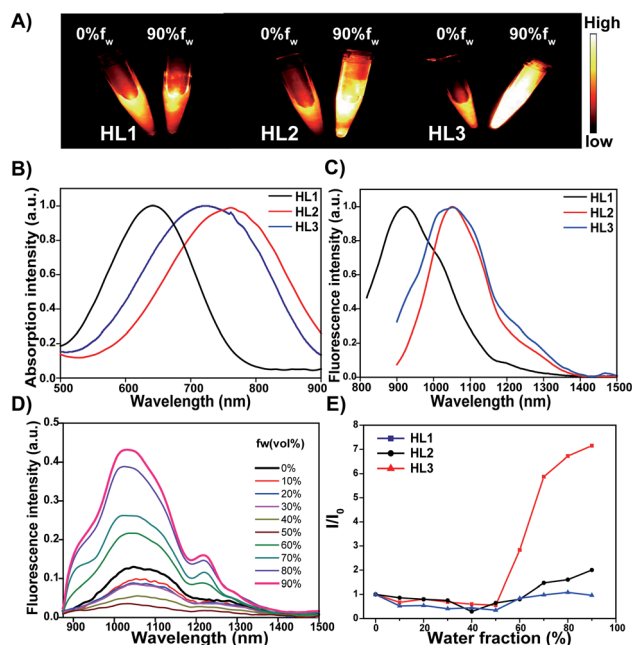
Fig. 3 (A) NIR-II fluorescence images (1000 LP, 808 nm excitation, 40 \text{mW cm}^{-2} , and 5 ms) of HL1–HL3 in THF and THF/water ( f_w 90%); (B) absorption and (C) fluorescence emission spectra of HL1–HL3 in THF under 808 nm excitation; (D) fluorescence emission spectra of HL3 obtained upon increasing f_w from 0 to 90% under 808 nm excitation; (E) fluorescence intensity ratios ( I/I_0 ) of HL1–HL3 in different f_w s, I_0 is the fluorescence intensity of HL1–HL3 in THF.
