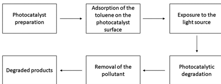
Fig. 3 Working procedure of the photocatalysts for toluene degradation.
