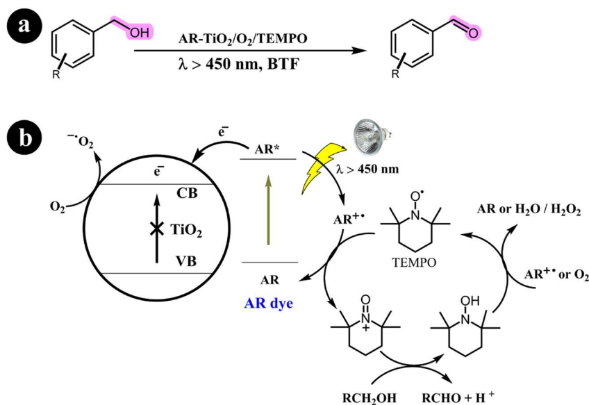
Scheme 2 The illustration of (a) the conversion of alcohols to their corresponding aldehydes and ketones and (b) the catalyst design and working mechanism. Reproduced with permission from ref. 36. Copyright 2008, John Wiley and Sons.
